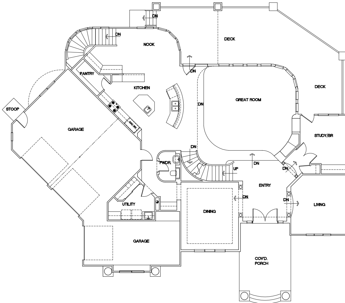
MAIN FLOOR PLAN 2402 S.F.
